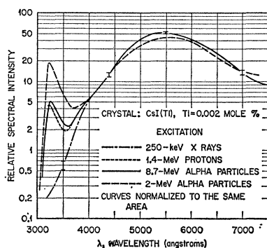
FIG. 1. Emission spectra of a CsI(Tl) crystal having a Tl content of 0.002 mole %, upon excitation by various radiations. Curves for 250-keV x rays, 1.4-MeV protons, and 8.7-MeV alpha particles are indistinguishable above 4000 Å.
