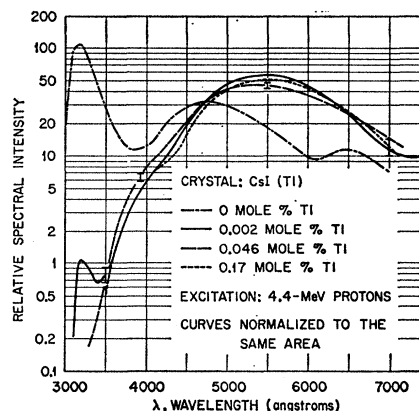
FIG. 3. Emission spectra of CsI(Tl) crystals having various Tl contents for excitation by 4.4-MeV protons.
